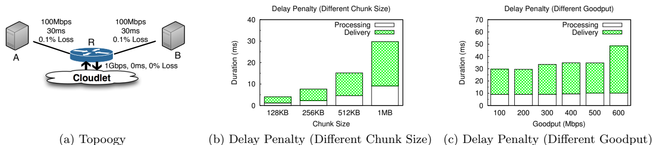
Figure 4: Evaluation on Deterlab
